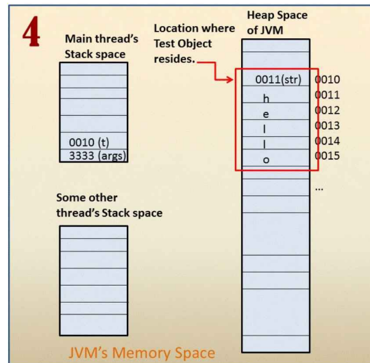
Step 4 - i and this are removed from the stack
