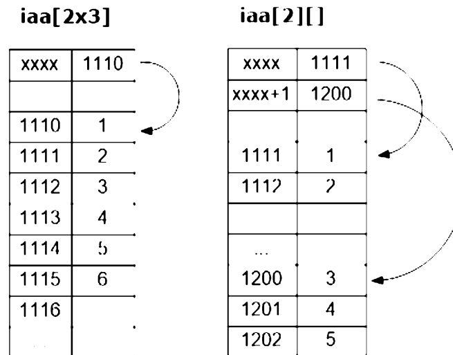
Rectangular vs Jagged arrays
