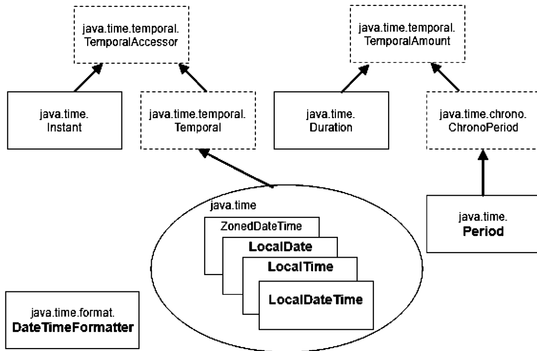
Organization of the new Date/Time API
