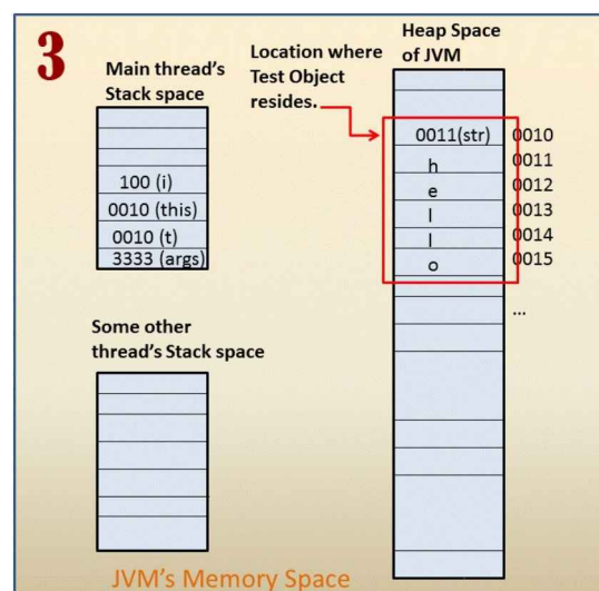
Step 3 - Two more variables i and this are added to the stack
