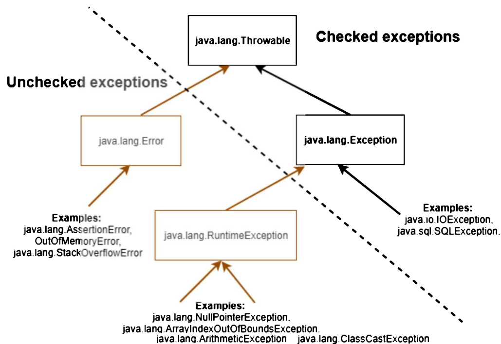
Checked and unchecked exceptions
