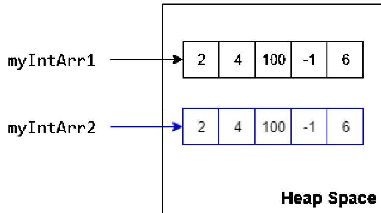
Cloning an array of ints
