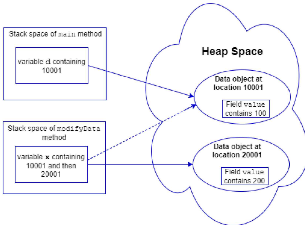
Passing an object to a method 2
